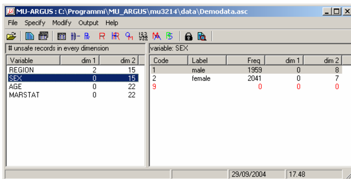
Figure 8. Output window for the individual risk methodology (2 sets of 2 key variables)
