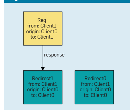
Figure 7. A simulated instance.
