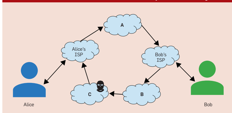
Figure 3. The attacker can only observe traffic going through autonomous system C, which allows him to monitor traffic from Bob to Alice and learn they are communicating.
