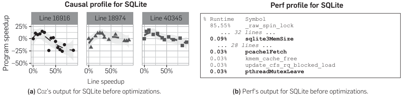
Figure 4. Coz and perf output for SQLite before optimizations. The three lines in the causal profile correspond to the function prologues for sqlite3MemSize , pthreadMutexLeave , and pcache1Fetch . A small optimization to each of these lines will improve program performance, but beyond about a 25% speedup, Coz predicts that the optimization would actually lead to a slowdown. Changing indirect calls into direct calls for these functions improved overall performance by 25.6\% \pm 1.0\% . While the perf profile includes the functions we changed, they account for just 0.15% of the sampled runtime.
