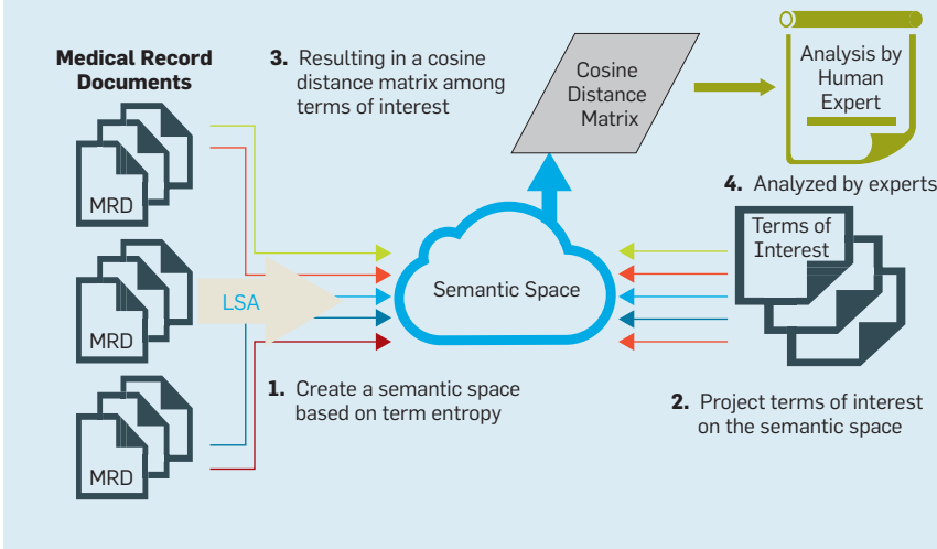
Figure 3. Outline of the latent semantic analysis process.
