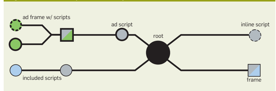
Figure 2. Generic example of a causality tree.
