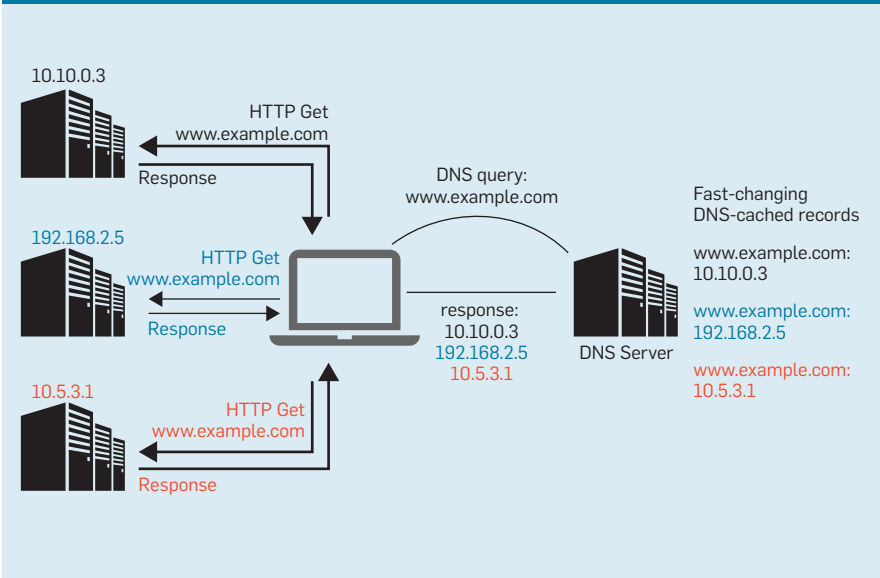
Figure 2. Fast flux.
