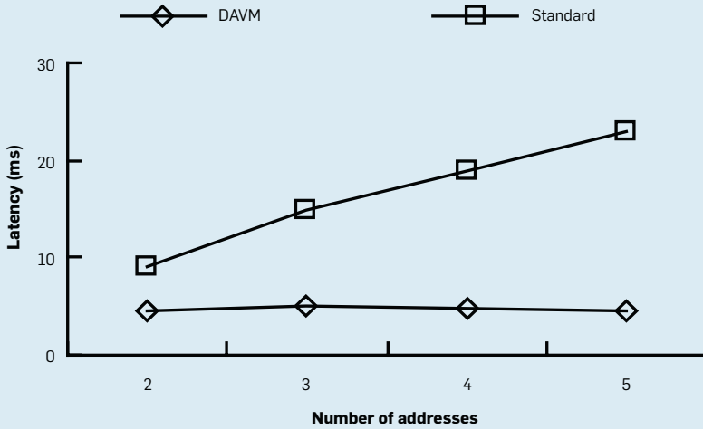
Figure 4. Addressing latency.
