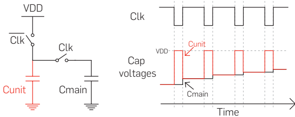
Figure 3. Design concepts of analog trigger circuit based on capacitor charge sharing.
