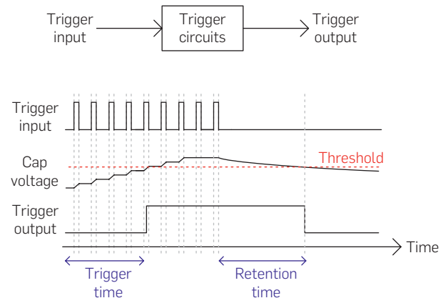
Figure 2. Behavior model of proposed analog trigger circuit.
