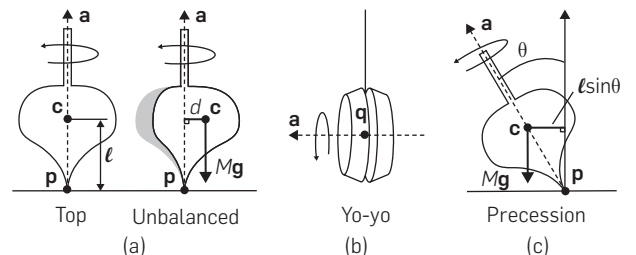
Figure 2. Spinning yo-yos and tops stably: for spinning tops, the center of mass must lie on the user-specified spinning axis a , otherwise it will cause an unbalanced external torque |\tau| = Mg d relative to p (a). For slower angular velocities, the precession angle \theta between rotational (vertical axis) and spinning axes becomes larger (c). For smaller \ell , the gravitational torque |\tau| = Mg \ell \sin \theta is smaller for equal precession, resulting in a longer spin. For yo-yos, we require the center of mass to coincide with q (b).
