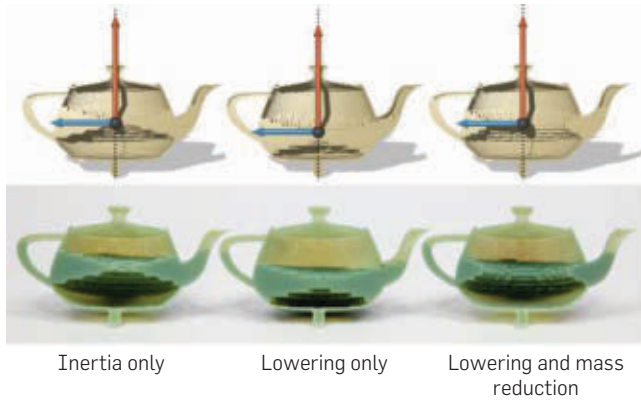
Figure 6. “Teapot”: (Left) Hollowed result showing voxelized interior mass and aligned axes using f_{\text{top}} = f_{y_0-y_0} . (Middle) Lowering of the center of mass shifts the mass distribution closer to the contact point. If we include mass reduction (right), mass is reduced inward out, resulting in the design with highest rotational stability.
