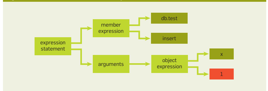
Figure 4. AST of one command in the corpus. (checking on this)
