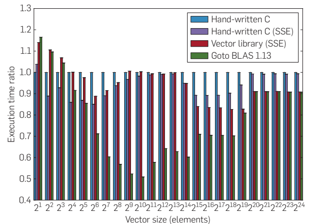
Figure 3. Relative performance of single-threaded ddot implementations. All times are normalized relative to the handwritten, compiler-vectorized, and C implementation.
