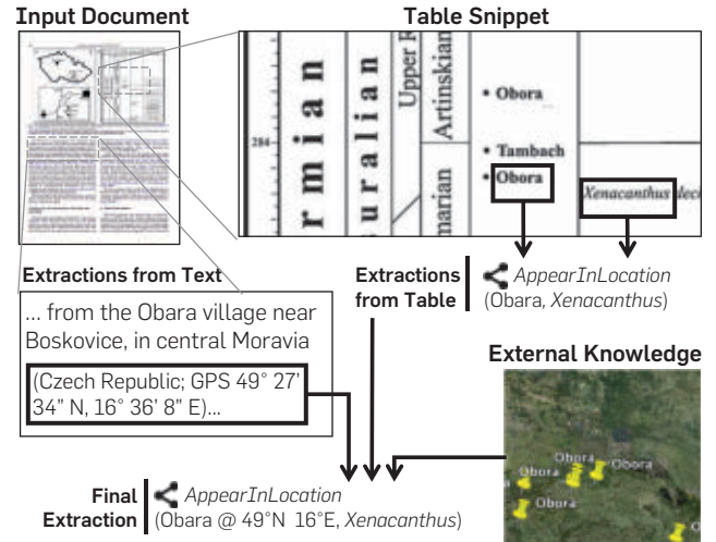
Figure 4. One challenge of building high-quality KBC systems is exploiting diverse sources of information jointly to extract data accurately. In this example page of a Paleontology journal article, identifying the correct location of Xenacanthus requires integrating information from within tables, text, and external structured knowledge bases. This problem becomes even more challenging when many extractors are not 100% accurate, motivating the joint probabilistic inference engine inside DeepDive.
