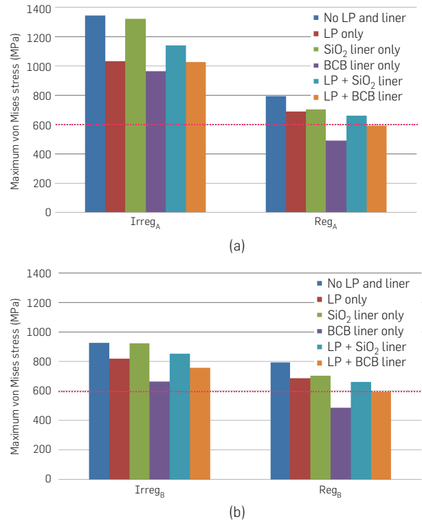
Figure 7. Impact of TSV structure, TSV placement style, and KOZ size on the maximum von Mises stress. (a) Designs with TSV A cell (KOZ = 1.205 μm) and (b) those with TSV B cell (KOZ = 2.44 μm).
