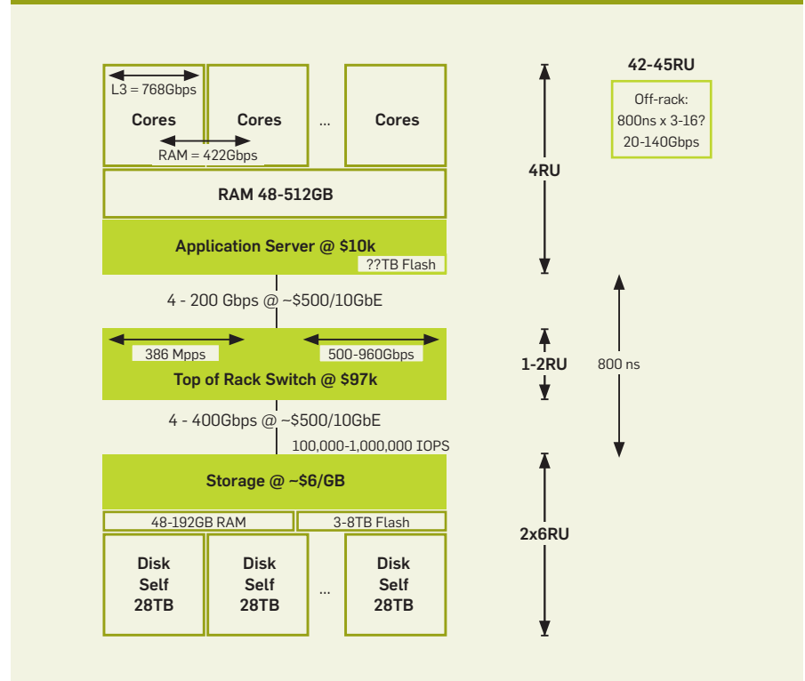
Figure 1. Enterprise rack diagram (ballpark list prices and specs are compiled from public data sources).
