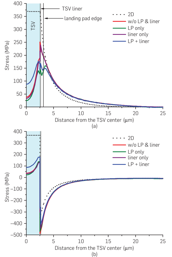
Figure 4. Effect of TSV structures on normal stress components. (a) \sigma_{rr} stress; (b) \sigma_{\theta\theta} stress.
