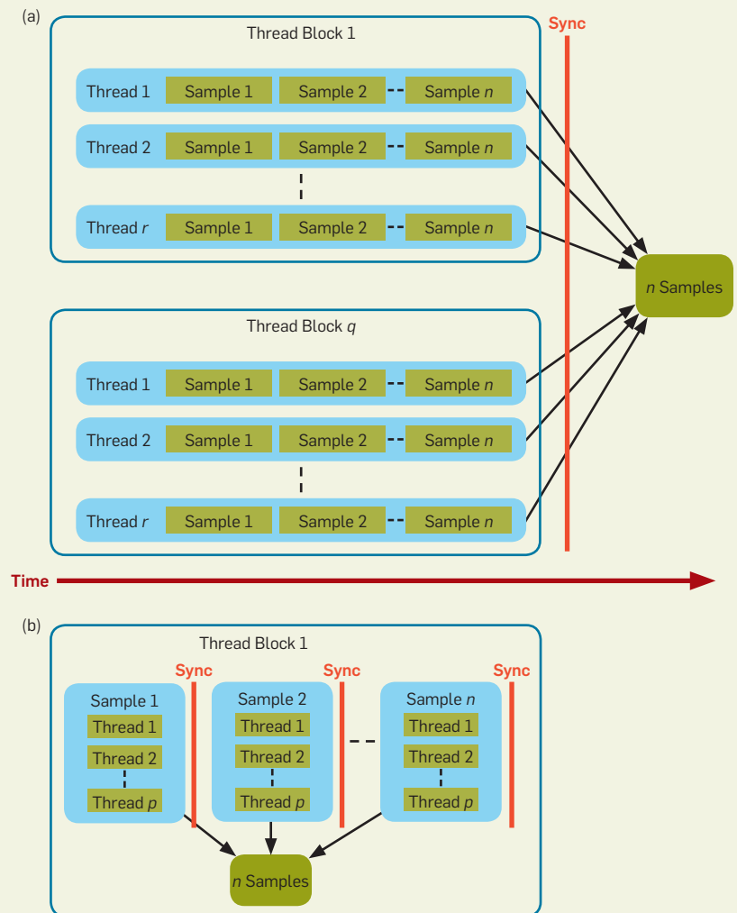
Figure 7. Two types of parallel audio applications.
