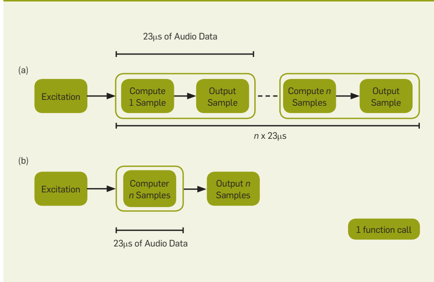
Figure 1. Real-time audio-synthesis approaches.
