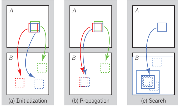
Figure 5. Phases of the randomized nearest neighbor algorithm: (a) patches initially have random assignments; (b) the blue patch checks above/green and left/red neighbors to see if they will improve the blue mapping, propagating good matches; (c) the patch searches randomly for improvements in concentric neighborhoods.
